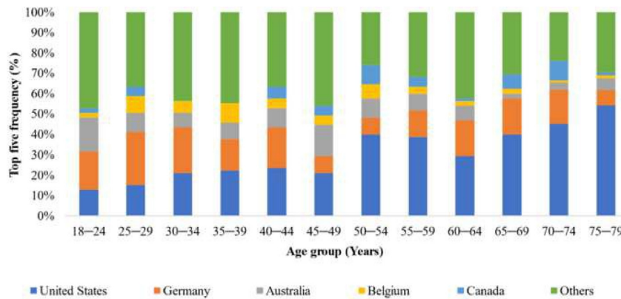
Fig. 2. Nationality frequency of top five male finishers in “Ironman Hawaii” by each age group for the male athletes.
